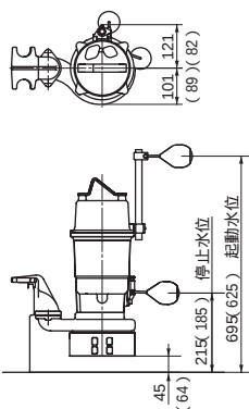
AH502D
