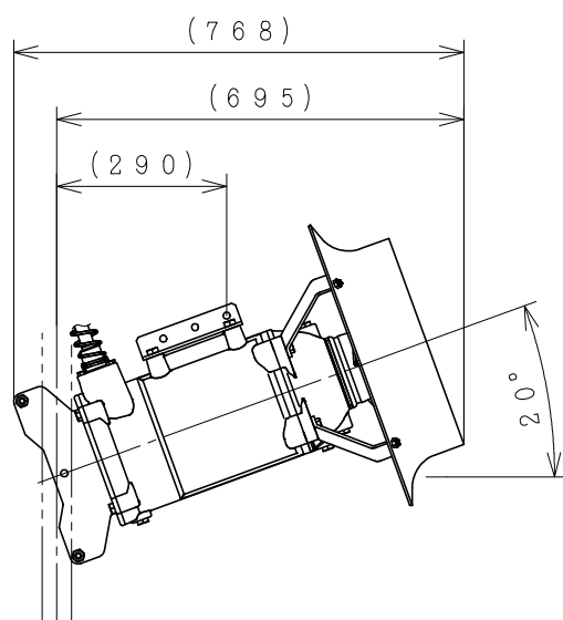
斜め上向き設置時 Obliquely upward installation
