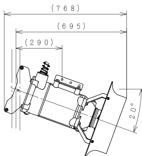
斜め下向き設置時 Obliquely downward installation
