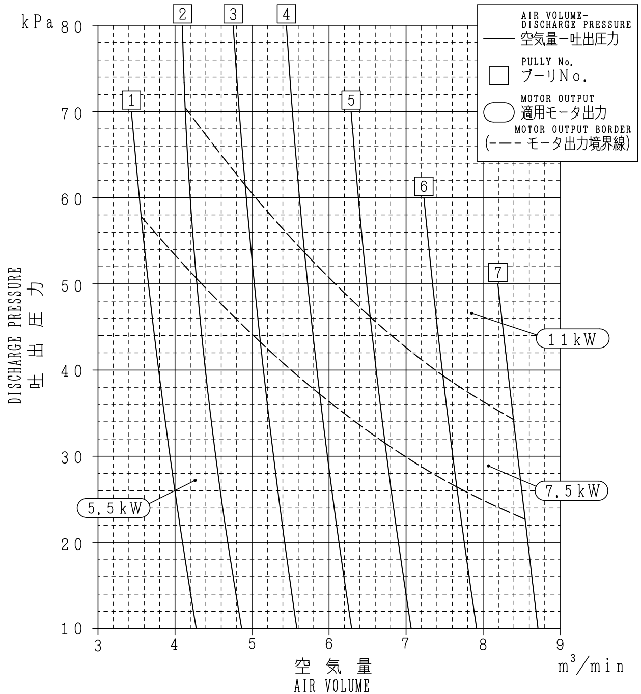
ARH100EX 性能曲線図 (PERFORMANCE CURVE)
